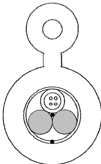
Fig. 3-1 Cross-section view of optical fiber three loose tubes stranded, dry core aerial fiber optic cable.
